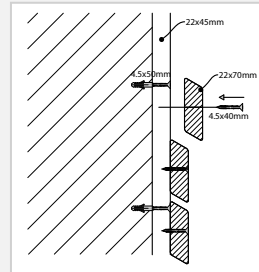
grenen 22 x 70 mm
