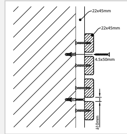
grenen 22 x 45 mm
